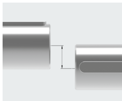
Max. radial displacement \Delta K_r
